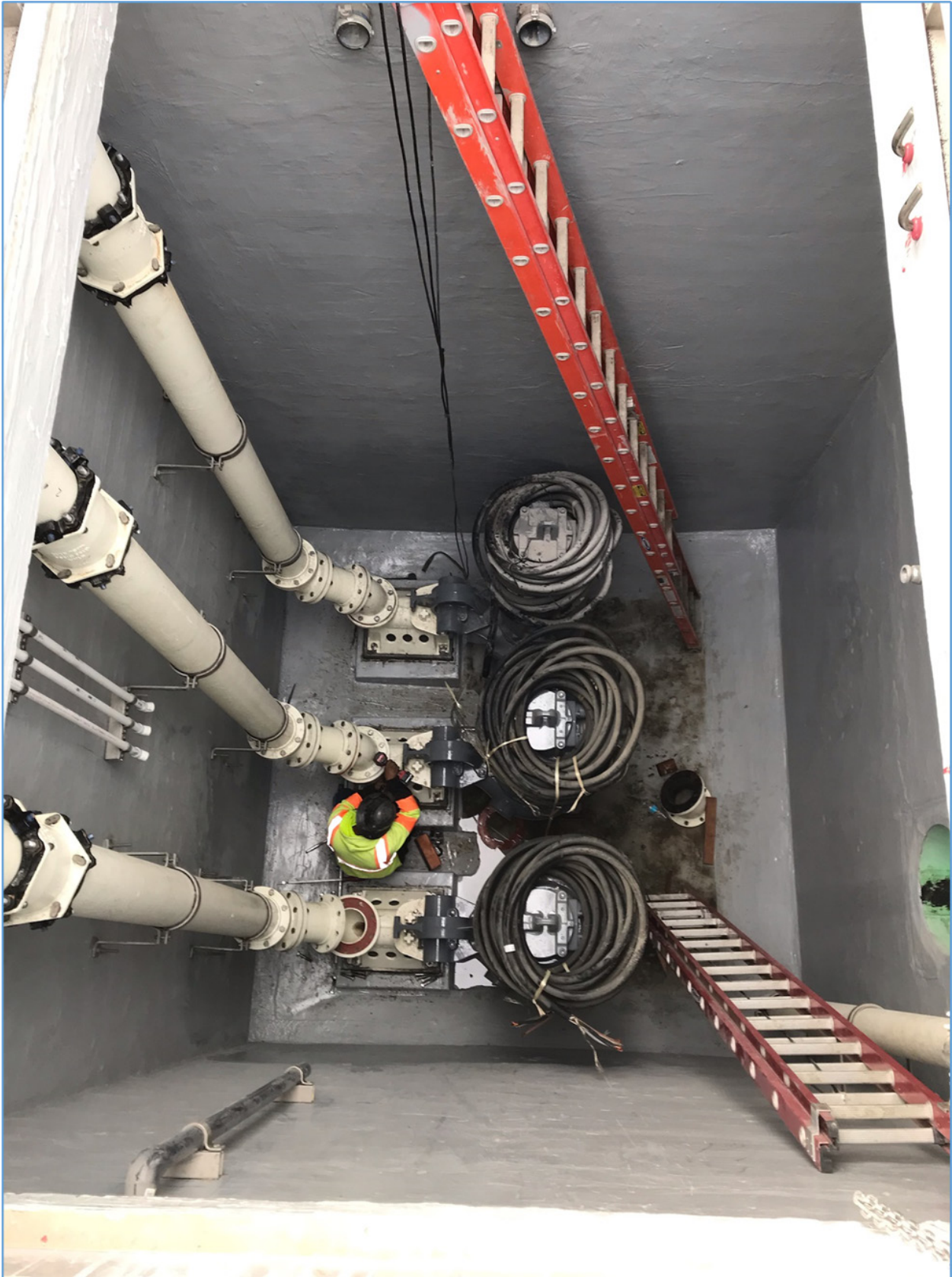
September 16, 2022 – Installing Piping and Pumps at Pump Station B Wet Well.
