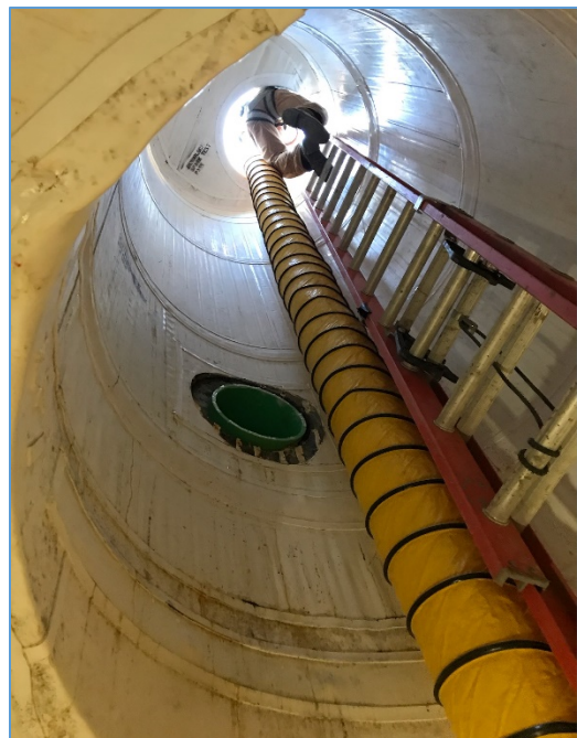
September 16, 2022 – Sealing Leaks and Holiday Testing Liner in Pump Station A Emergency Storage Tanks.
