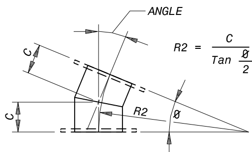
2-PIECE ELBOW 0-30° (0-0.52 rad)
