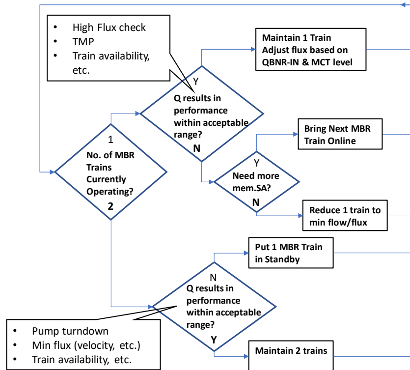
Figure 3-4.02.01. Overview of MBR System Basin Operation Management
