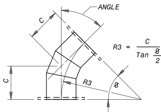
3-PIECE ELBOW 31-60° (0.54-1.0 rad)
